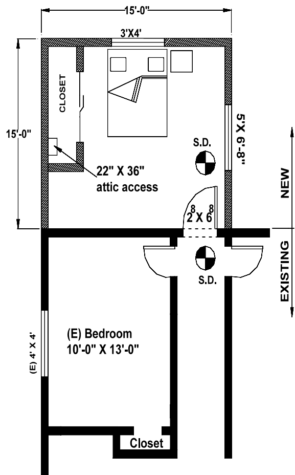
Floor Plan
