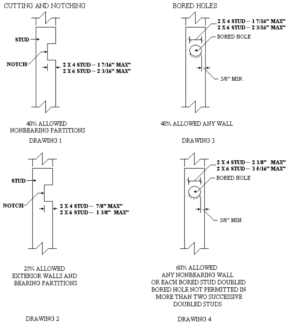
Figure 6: Maximum Allowed Notching and Drilling for Normal Construction with 2x Studs
