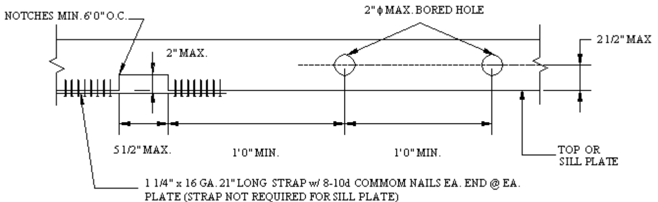
2 x 6 DBL. TOP PLATE, 2 x 6 or 3 x 6 SILL PLATE
