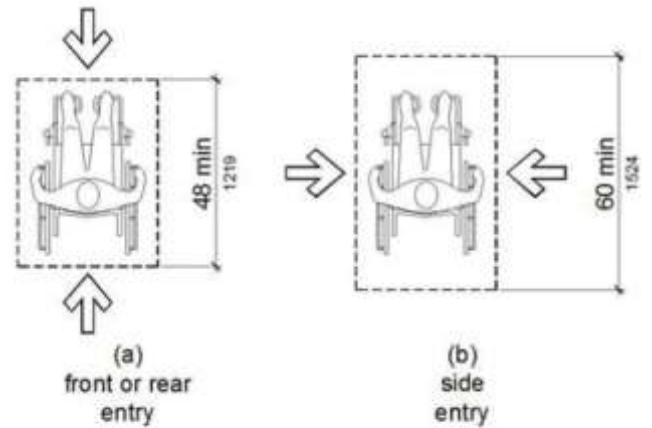
FIGURE 11B-802.1.3 DEPTH OF WHEELCHAIR SPACES
