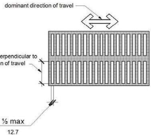
FIGURE 11B-302.3 ELONGATED OPENINGS IN FLOOR OR GROUND SURFACES
