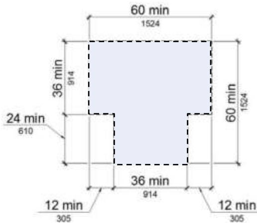
FIGURE 11B-304.3.2 T-SHAPED TURNING SPACE
