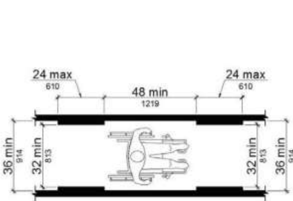
FIGURE 11B-403.5.1 CLEAR WIDTH OF AN ACCESSIBLE ROUTE
